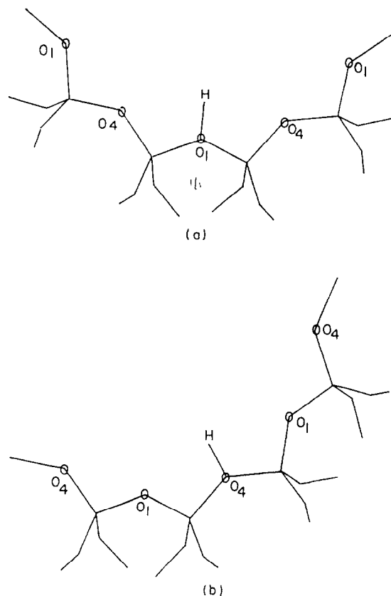
Fig. 5. The tetrameric cluster centered at O1 (FWC1) and O4 (FWC4) of zeolite H–Y framework are shown as structures (a) and (b), respectively. These cluster models represent the two possible Bronsted acid sites in 12 m ring of H–Y.
