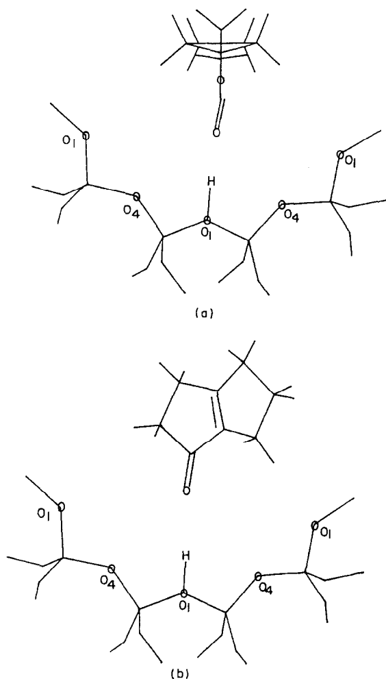
Fig. 6. The orientation of a typical spirolactone (1) and enone (6) molecules with respect to the zeolite framework cluster model shown in Fig. 5a. These cluster models are chosen to study the electronic interaction between the molecule and zeolite framework.
