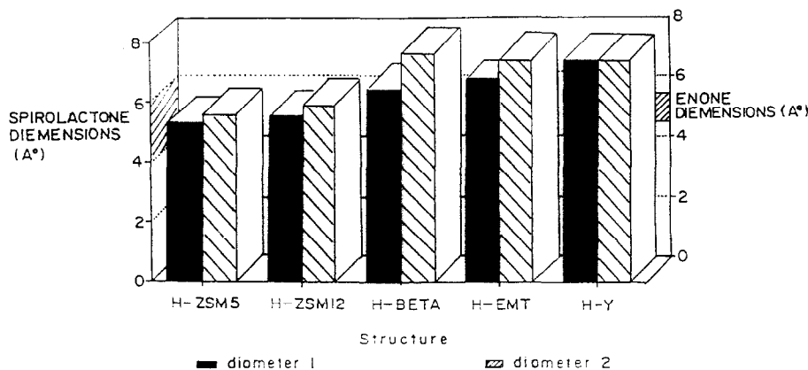
Fig. 3. The schematic representation of the pore diameters in various zeolites used as catalysts. The diameters of two pores in case of 2D pore structures or the two diameters of elliptical 1D pore structures are shown. The range of smallest dimension of the reactant spirolactone and product enone molecules are indicated as shaded regions. The actual dimensions are given in Table 1.
