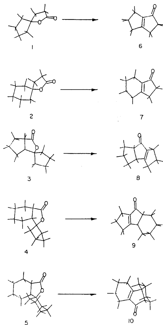
Fig. 1. The 3D structure of spirolactone and enone molecules, as derived from force field calculations.
